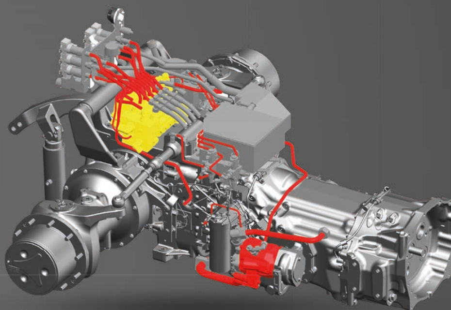
Lintrac 130
